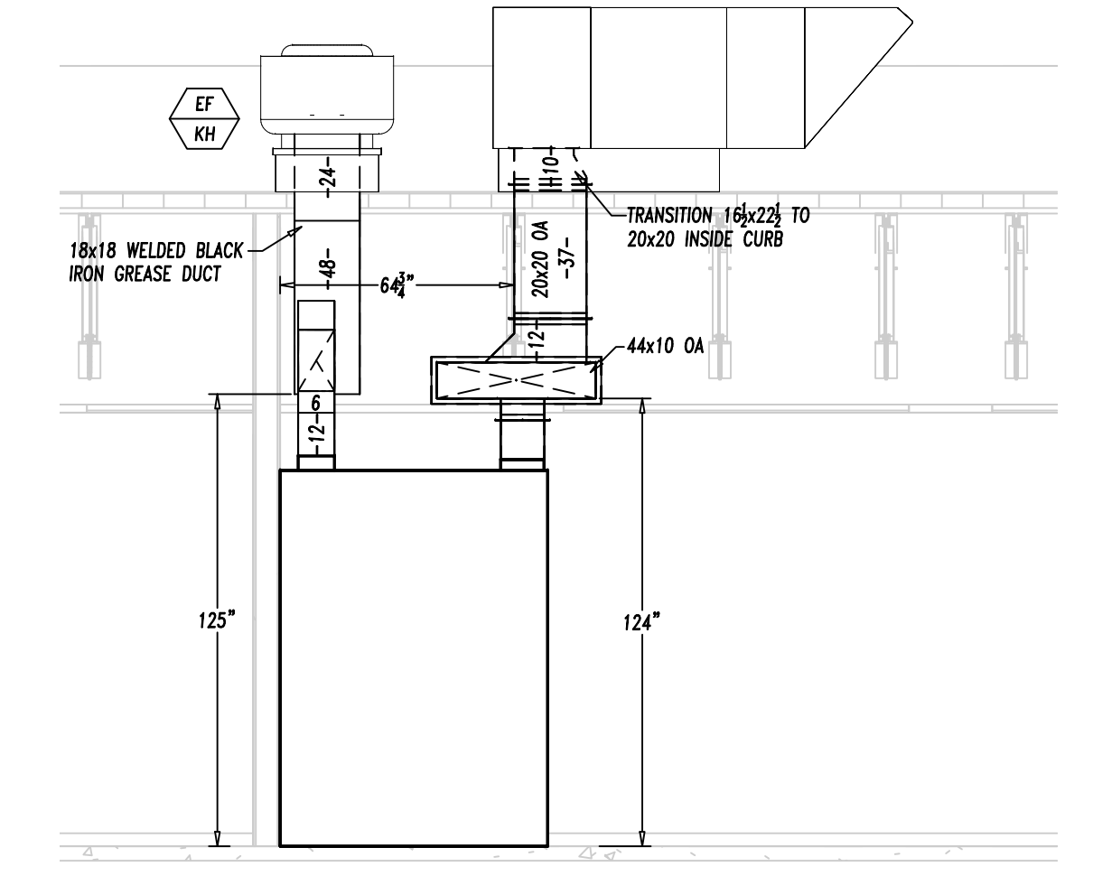
6 EF-KH & MAU-1 SECTION VIEW SCALE: 1/4" = 1'-0"
